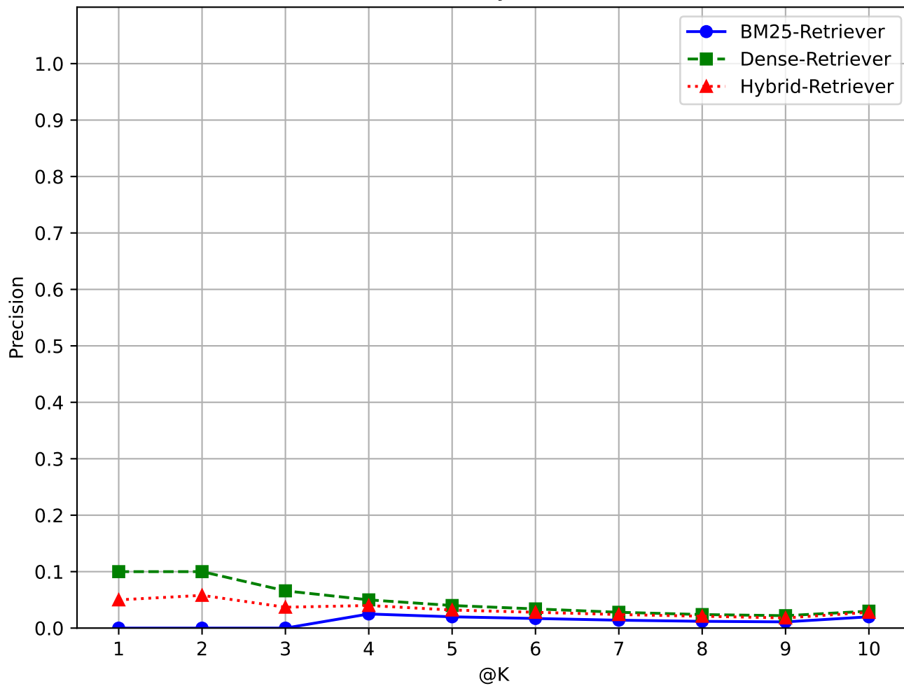
Query 39
